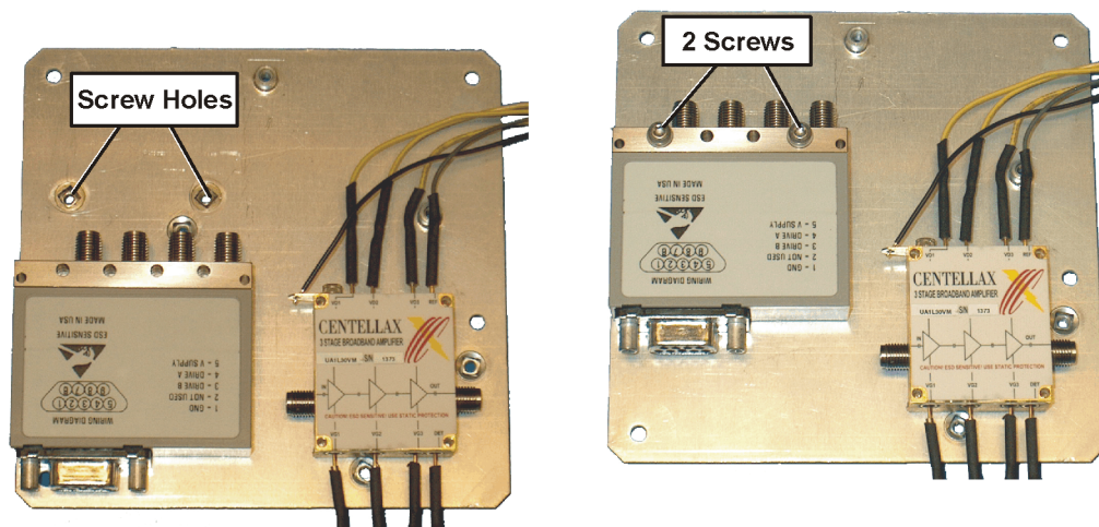
Figure 13 Attaching RF Switch to Bracket
