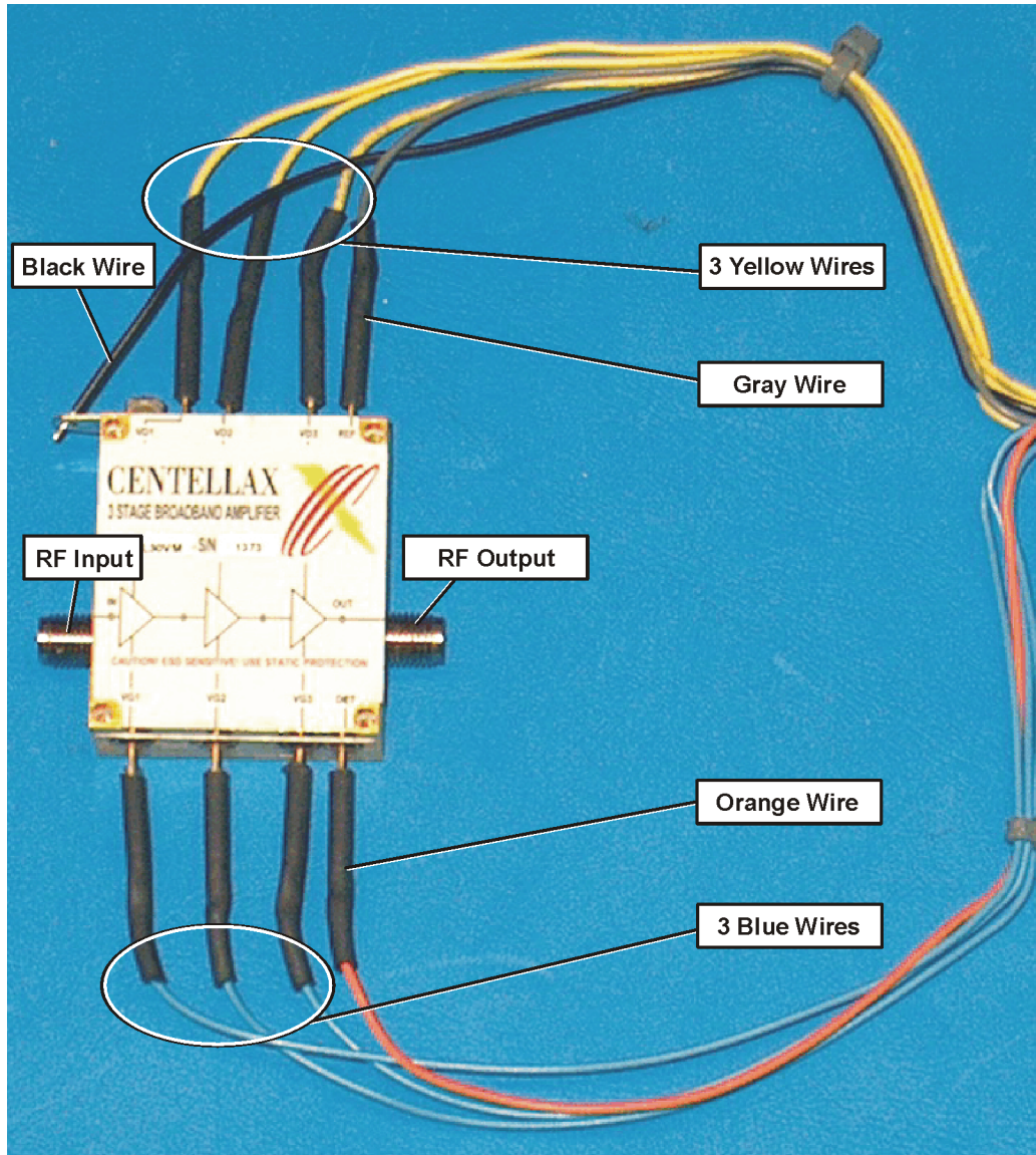
Figure 11 Attaching the Cable Assembly to the Amplifier
