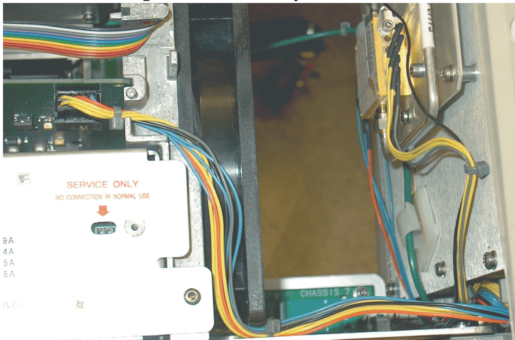
Figure 20 Dressing the Cable Assembly
