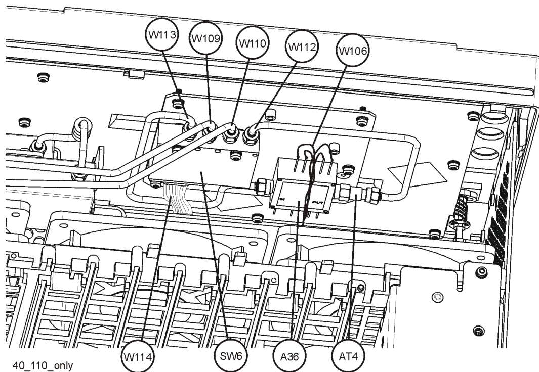
Figure 21 Option 110 Assemblies and Cables
