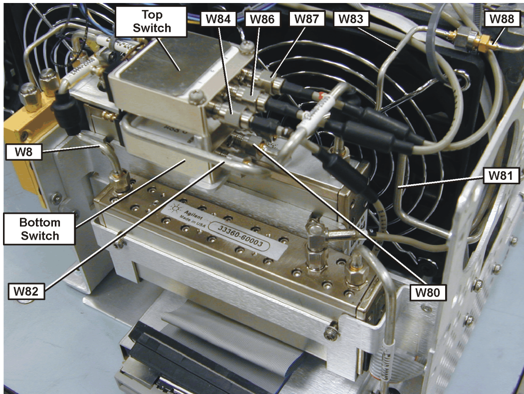
Figure 22 Option 123 Assemblies and Cable Locations
