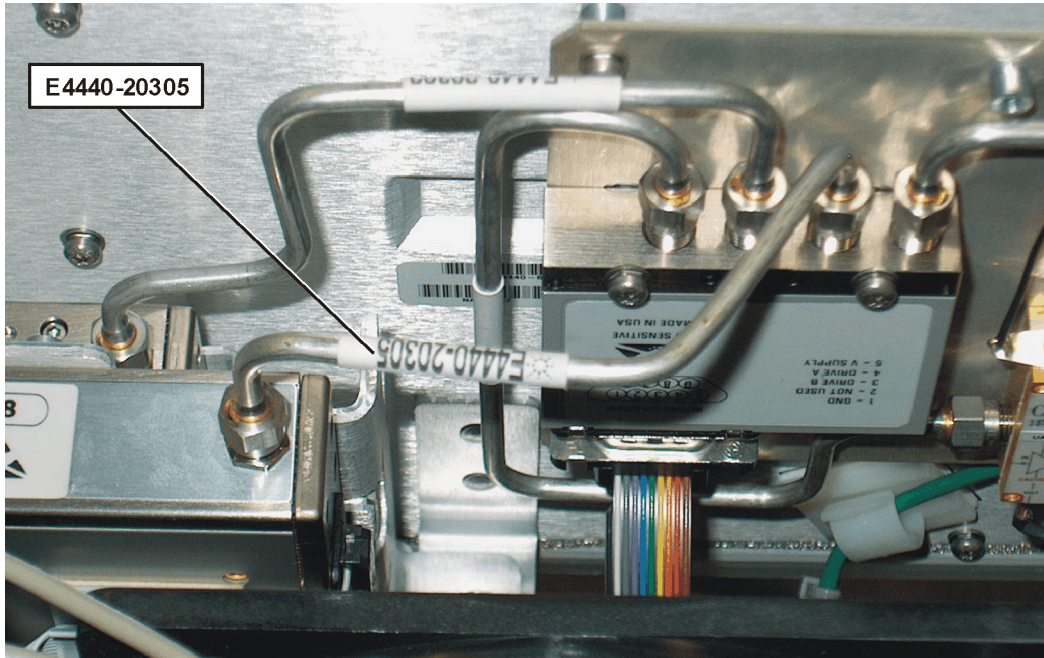
Figure 5 Removing the E4440-20305 Cable
