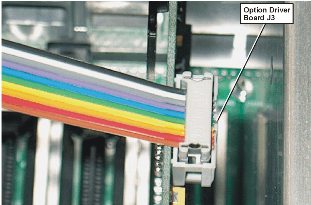
Figure 19 Ribbon Cable Connected to J3
