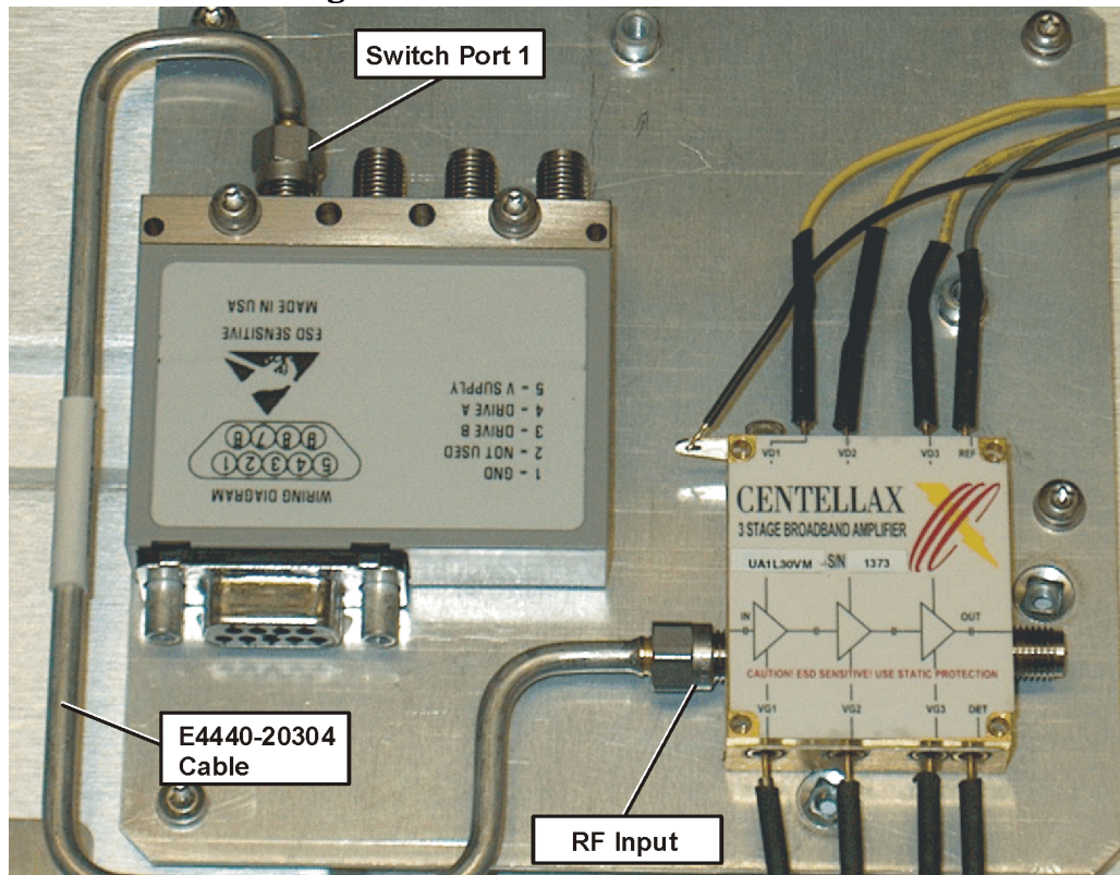
Figure 15 Attaching E4440-20304 cable
