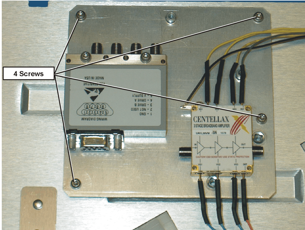
Figure 14 Installing the Bracket to the Front Frame
