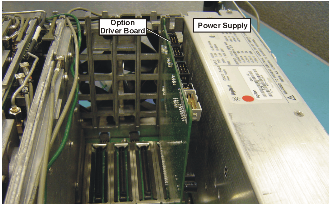
Figure 9 Option Driver Board Installation
