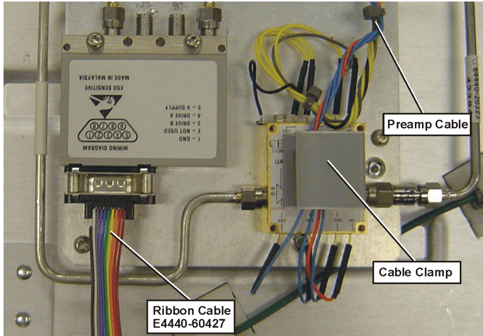
Figure 17 Installing Ribbon Cable and Routing Cable Assembly
