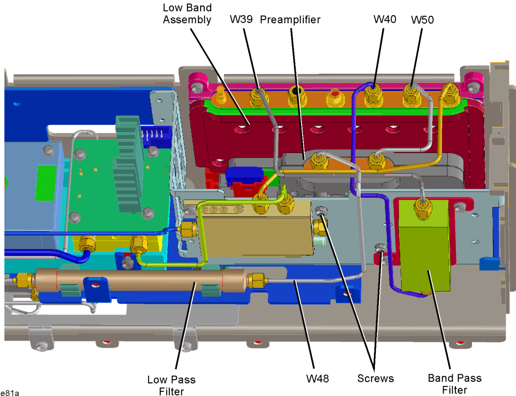
Figure 3 Preamplifier Location
