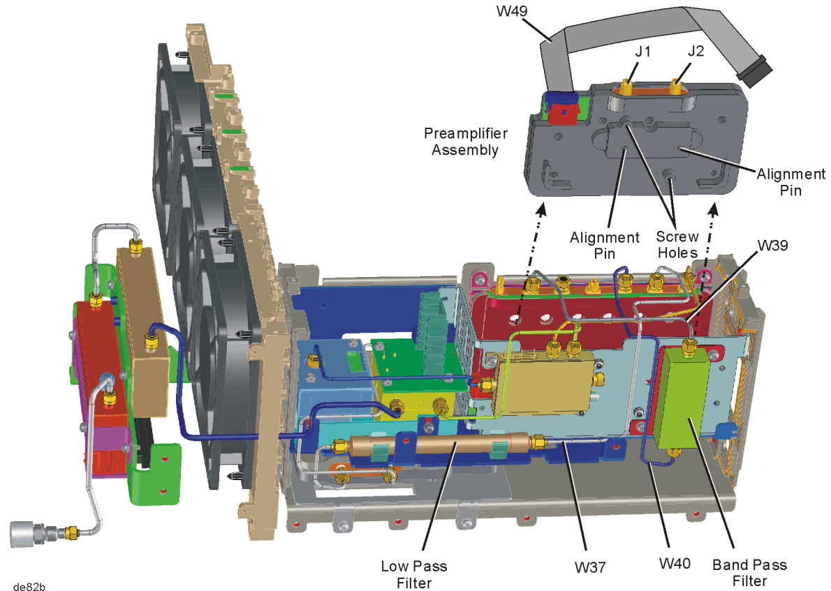
Figure 4 Remove the Preamplifier
