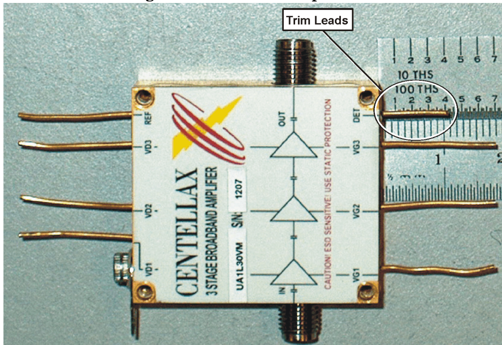
Figure 10 Trimming the Leads on the Amplifier
