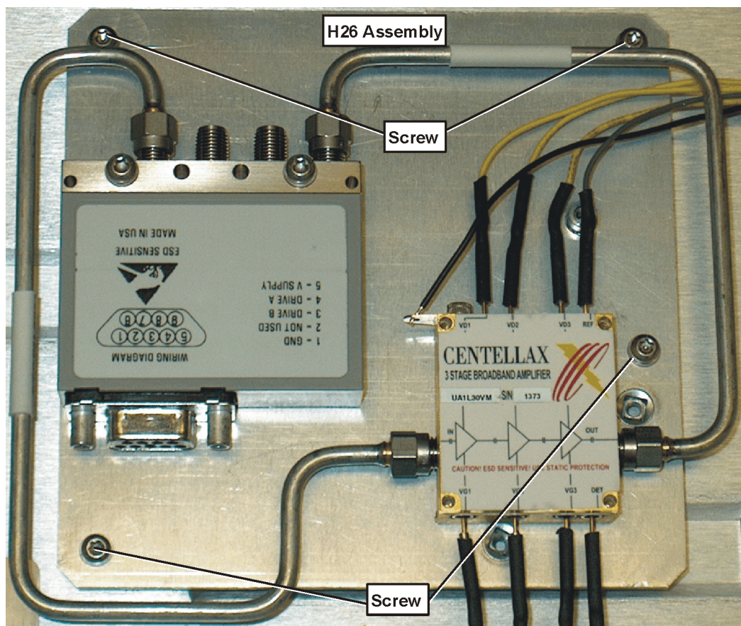
Figure 7 Removing the H26 Assembly
