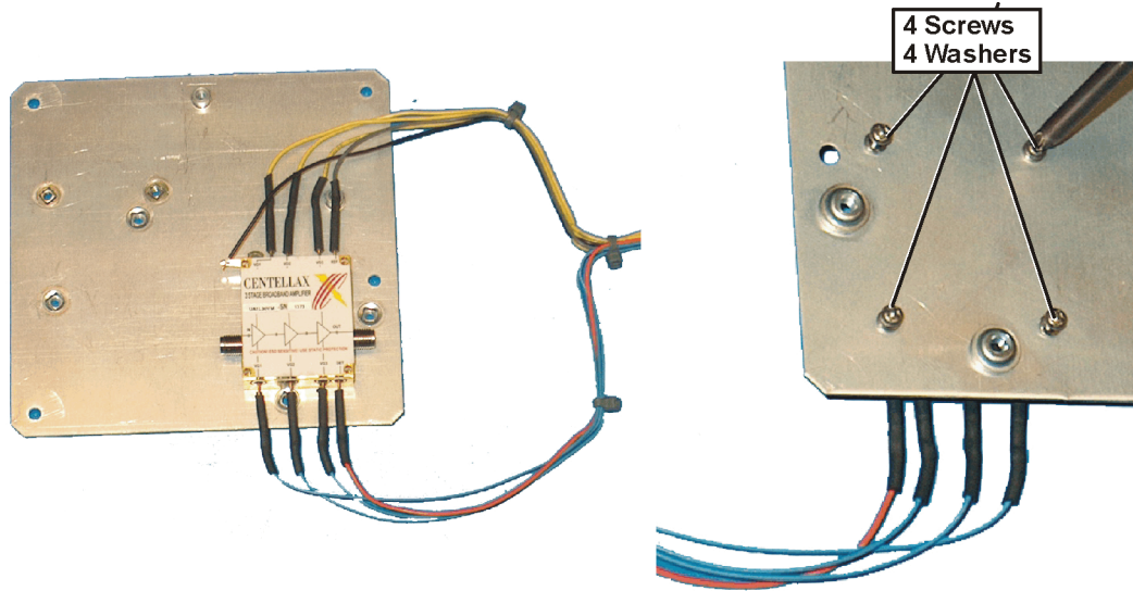
Figure 12 Installing the Amplifier
