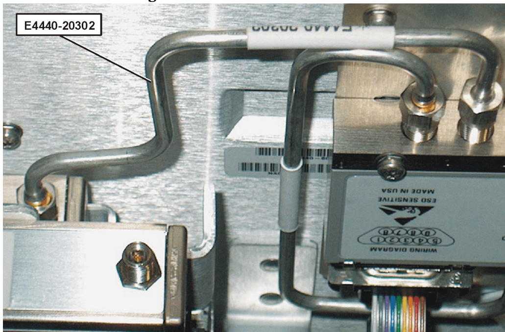
Figure 6 Removing the E4440-20302 Cable
