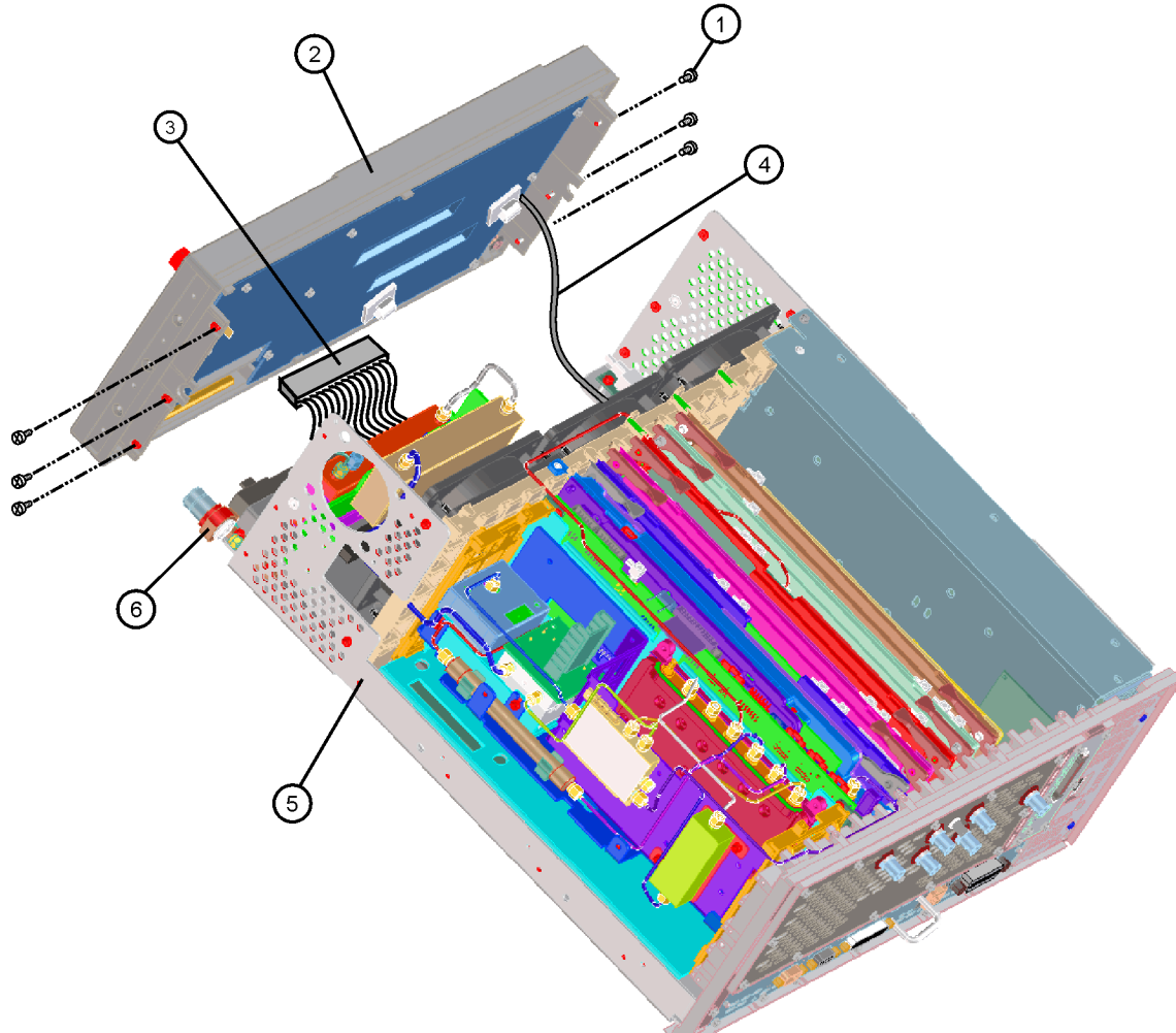
Figure 8 Front Frame Assembly Removal (6 PLACES)
