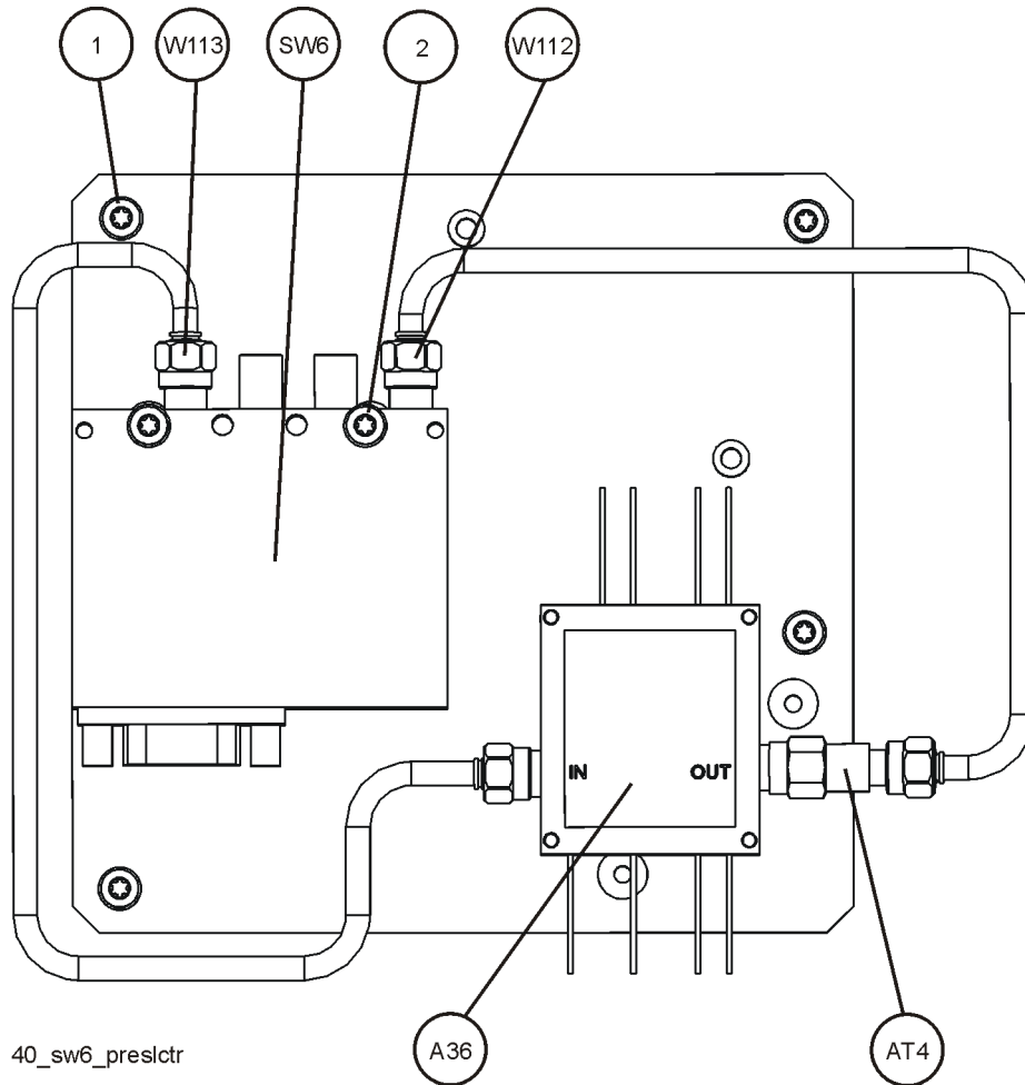
Figure 16 Option 110 A36 Preamplifier and Switch SW6
